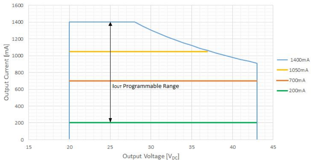
RTLD040-1400A-SA
