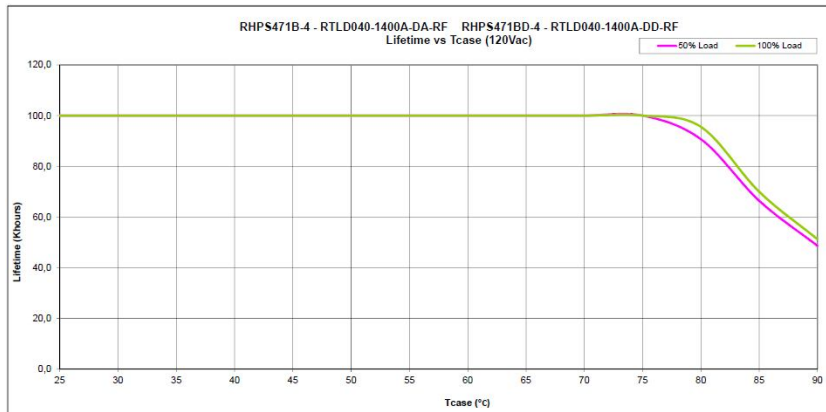
RTLD040-1400A 120 V AC Full/Half load
