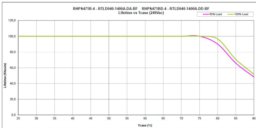
RTLD040-1400A 240 V AC Full/Half load
