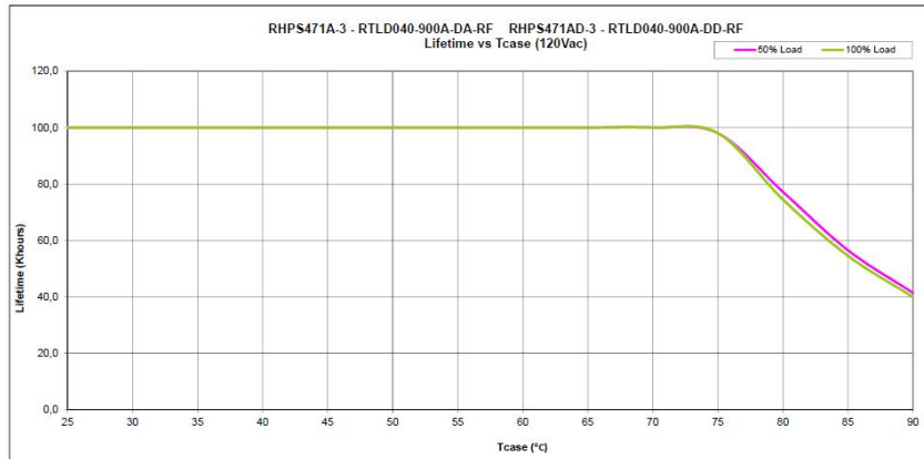
RTLD040-900A 120 V AC Full/Half load
