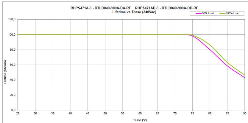
RTLD040-0900A 240 V AC Full/Half load
