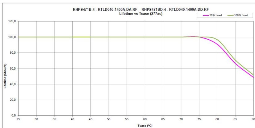
RTLD040-1400A 277 V AC Full/Half load
