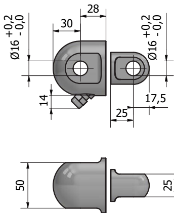
Alu/Stainless steel Max. static load 18100 N
